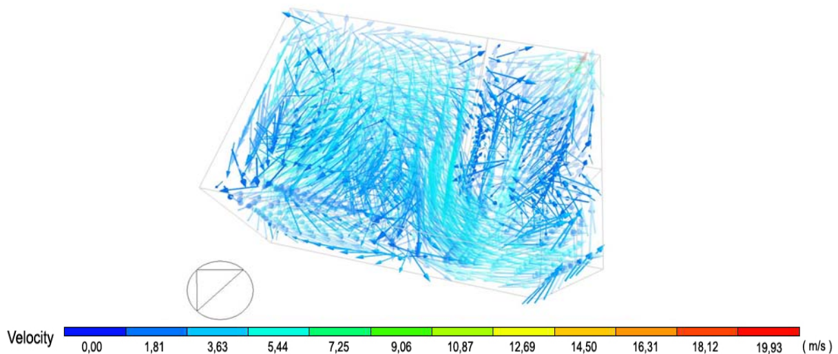
Figure 9. The simulation result in option 4 is illustrated for the velocity in the virtual model testing
