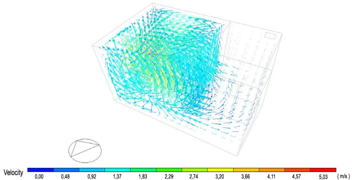
Figure 6. The simulation result in option 1 is illustrated for the velocity in the virtual model testing
