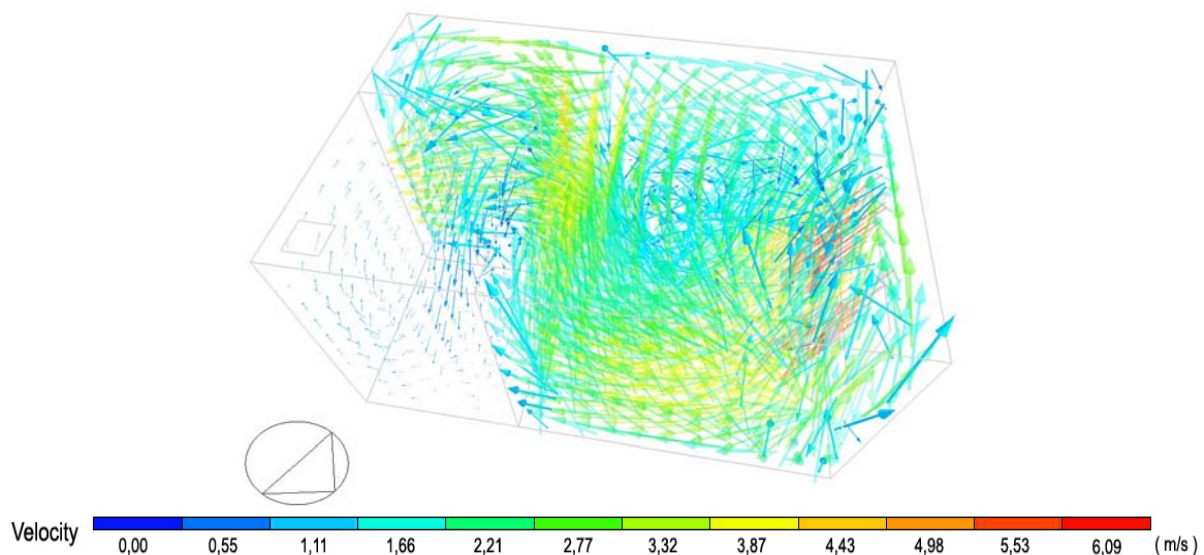
Figure 7. The simulation result in option 2 is illustrated for the velocity in the virtual model testing
