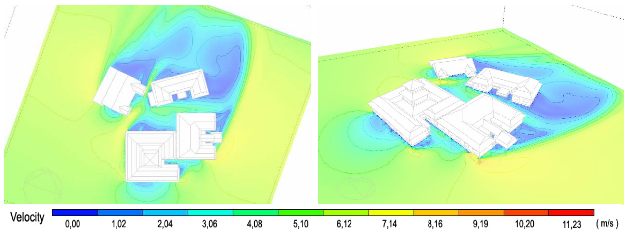
Figure 5. The simulation of the wind flow stream affect to whole building
