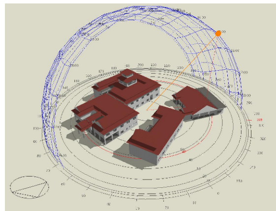
Figure 2. The software parameter inputs and the virtual model in CFD DesignBuilder
