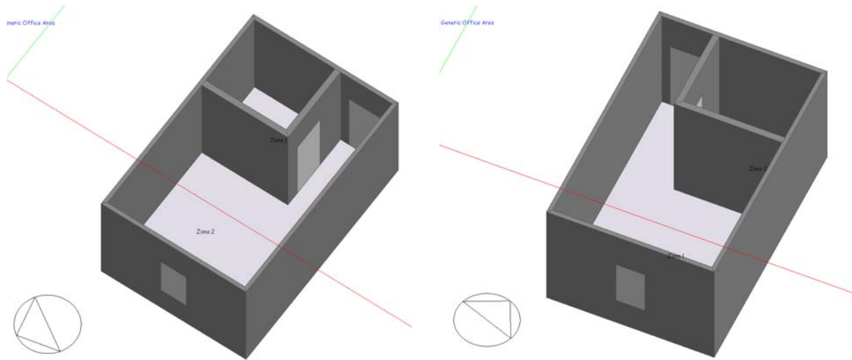
Figure 4. The virtual model for testing about the different position of the bathroom
